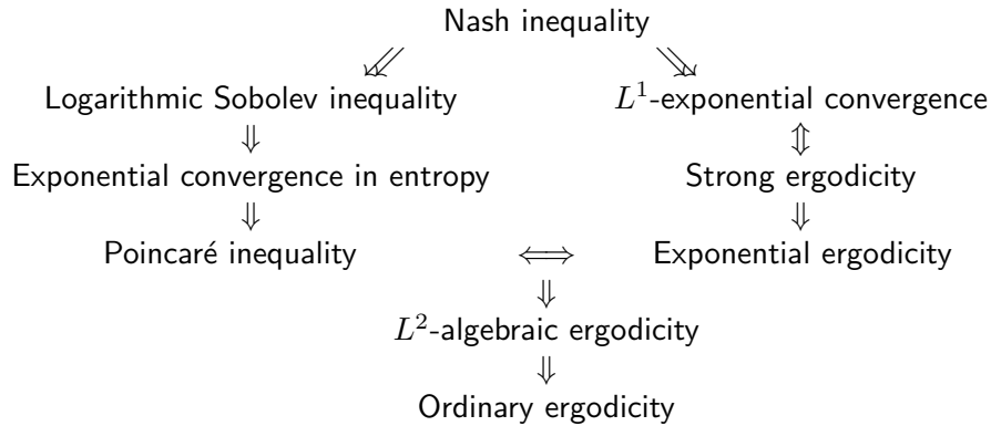
Figure 4.1 Diagram of nine types of ergodicity In Figure 4.1, L^2 -algebraic ergodicity means that
