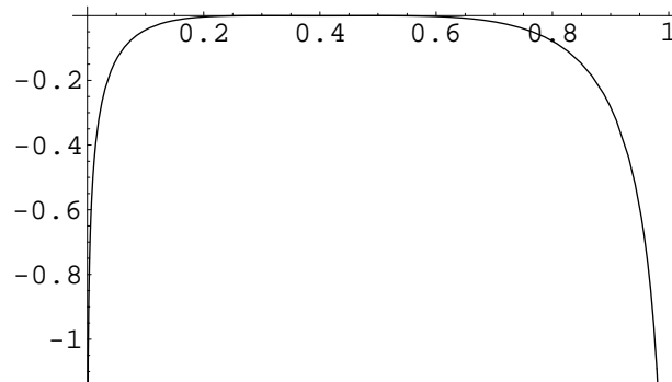
Figure 1: The picture of f_a(\cdot, 0.3) .
