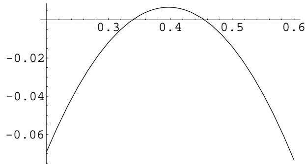
Figure 4: The picture of \partial_{xx}^2 f_a(\cdot, 0.3) on [0.2, 0.6] .
