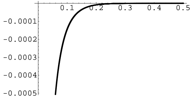
Figure 9: The graph of the function in (33).
