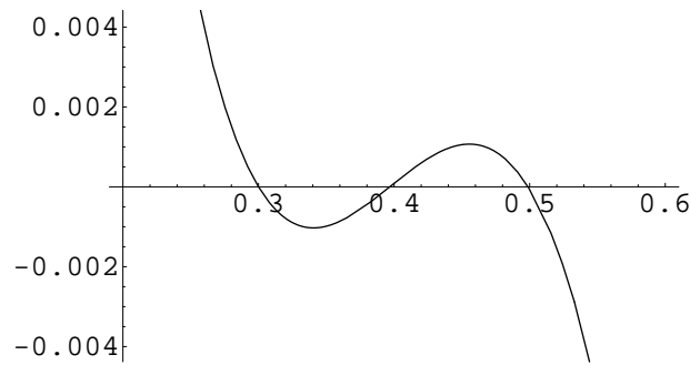
Figure 3: The picture of \partial_x f_a(\cdot, 0.3) on [0.2, 0.6] .
