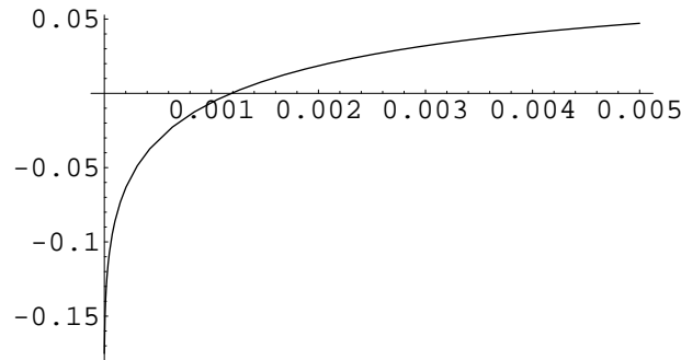
Figure 8: The graph of \partial_x f_a(x_2, \cdot) on (0, 0.05) .
