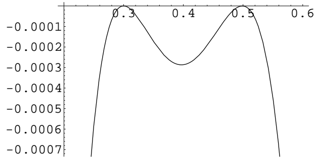
Figure 2: The picture of f_a(\cdot, 0.3) on the smaller interval [0.2, 0.6] .
