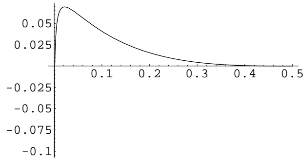
Figure 7: The graph of \partial_x f_a(x_2, \cdot) on (0, 0.5) .
