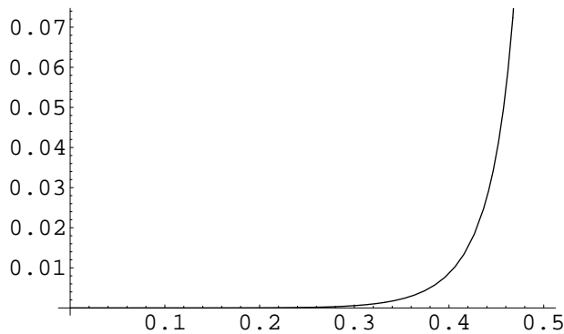
Figure 6: The graph of the function g in (30).
