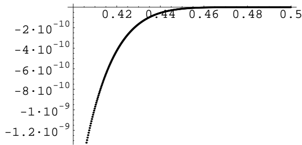
Figure 10: The graph of the function in (33) on [0.4, 0.5] .
