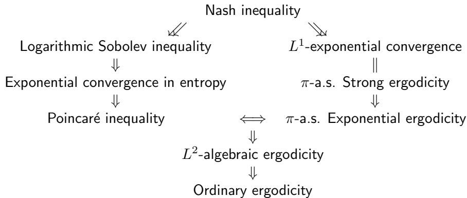
Figure 9.1 Diagram of nine types of ergodicity
