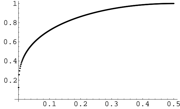
Figure 5: The graph of 2\alpha_1(\theta) - 1 .
